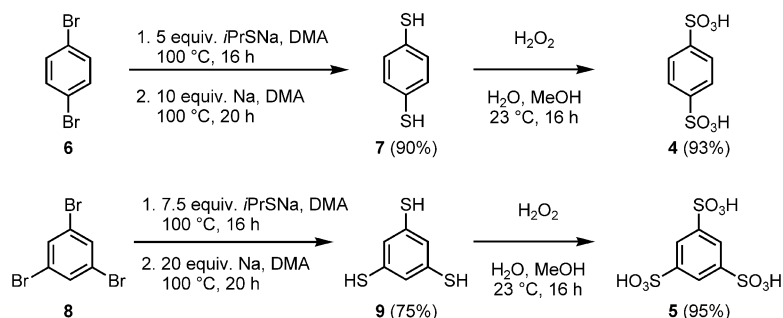
Scheme 1. Synthesis of sulfonic acids p -BDSH 2 ( 4 ) and BTSH 3 ( 5 ).
