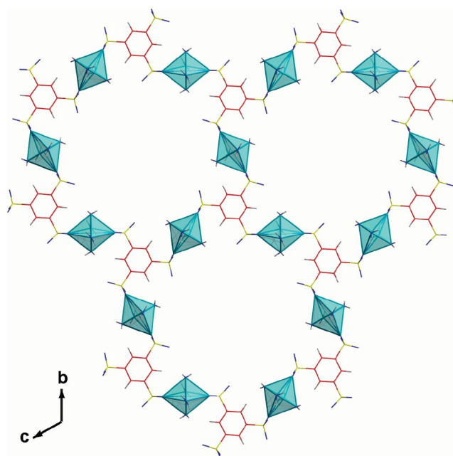
Figure 6. View onto a single layer of compound ( III ). Rotation ( 60^\circ ) and superposition of these layers generates the complete structure.
