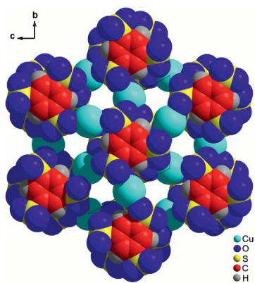
Figure 8. Space-filling representation of compound III , showing the open channels that permeate the solid down the a axis (solvent molecules are omitted).
