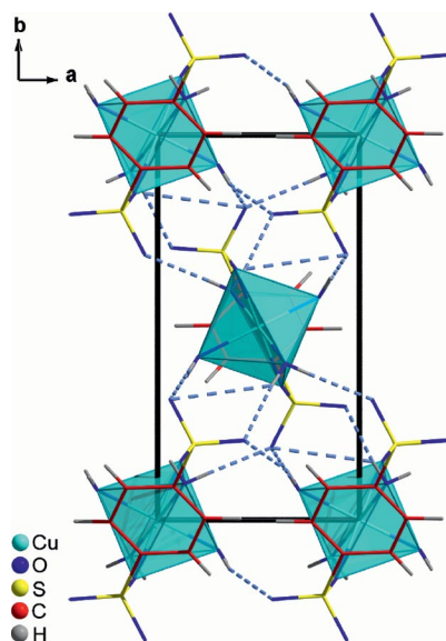
Figure 5. Projection of the crystal structure of [\text{Cu}(p\text{-BDS})(\text{H}_2\text{O})_4] ( II ) onto the (001) plane which shows the linkage of the chains to a 3D network through hydrogen bonds.
