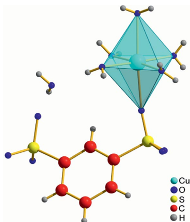
Figure 2. Typically distorted Cu 2+ polyhedron shown for [Cu( m -BDS)(H 2 O) 5 ]·H 2 O ( I ).
