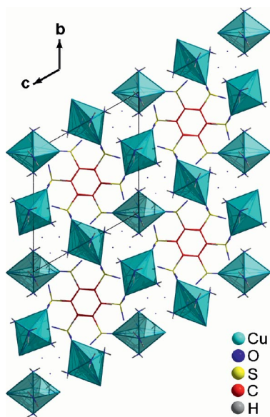
Figure 7. Projection of [\text{Cu}_3(\text{BTS})_2(\text{H}_2\text{O})_{12}] \cdot 6\text{H}_2\text{O} ( III ) onto the (100)-plane.
