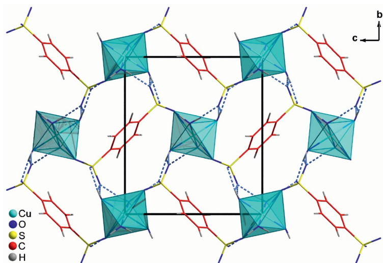
Figure 4. Connection of \text{Cu}^{2+} ions to form chains and formation of the network of [\text{Cu}(p\text{-BDS})(\text{H}_2\text{O})_4] ( II ) by hydrogen bonds (dashed lines) of the 1,4-benzene disulfonate linker.
