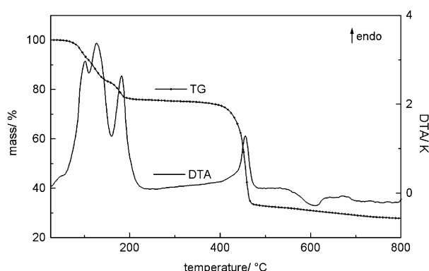
Figure 11. Thermal analysis of [\text{Cu}_3(\text{BTS})_2(\text{H}_2\text{O})_{12}] \cdot 6\text{H}_2\text{O} (III).
