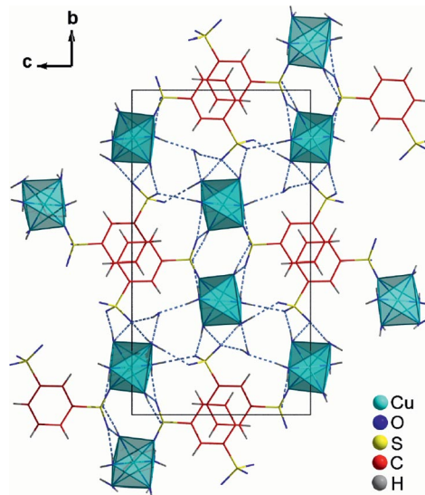
Figure 3. Projection of the crystal structure of [Cu( m -BDS)(H 2 O) 5 ]·H 2 O ( I ) onto the (100) plane. Hydrogen bonds are represented by dashed lines.
