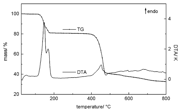
Figure 10. Thermal analysis of [\text{Cu}(\text{p-BDS})(\text{H}_2\text{O})_4] (II).
