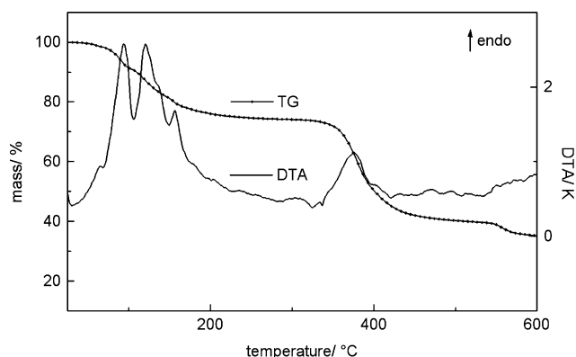
Figure 9. Thermal analysis of [\text{Cu}(m\text{-BDS})(\text{H}_2\text{O})_5] \cdot \text{H}_2\text{O} ( I ).
